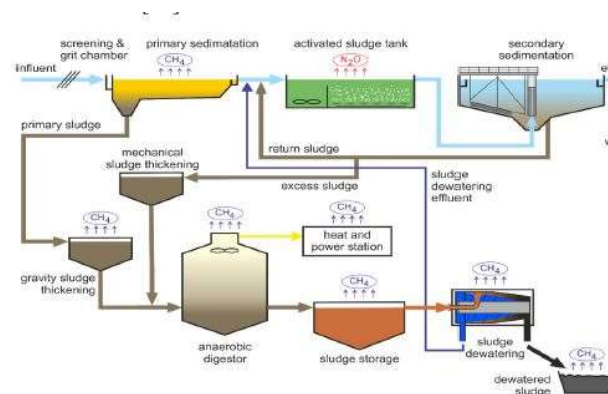
Figure 45 GHG Emissions at WWTP, Source : Parravicini et al. (2016)
