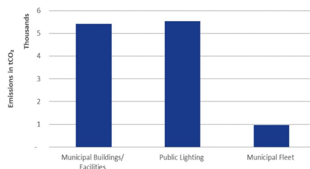
Figure 39 Emissions in tCO 2 by Sector in the Municipality
