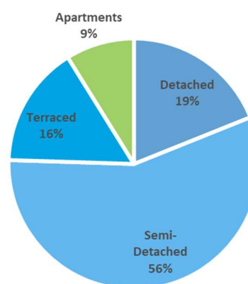
Figure 5 South Dublin's Residential Emissions by Dwelling Type
