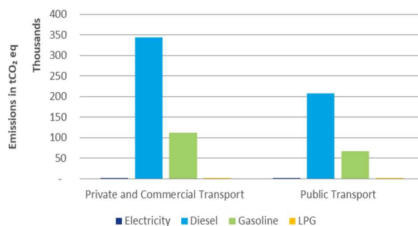
Figure 27 South Dublin's CO 2 Emissions From Transportation
